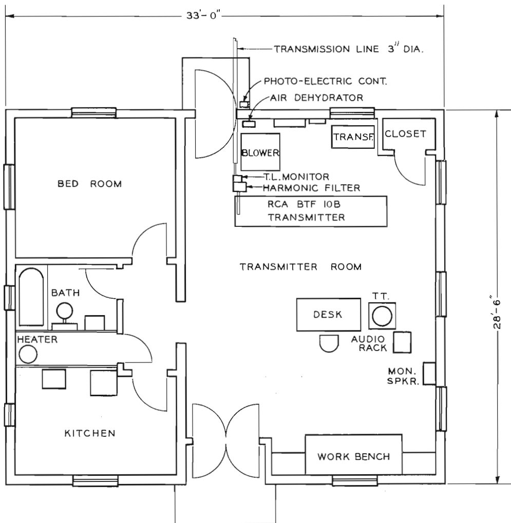
FIG. 8. The WKPT-FM transmitter building floor plan layout. All equipment is accommodated in a space approximately 30 feet by 30 feet.
