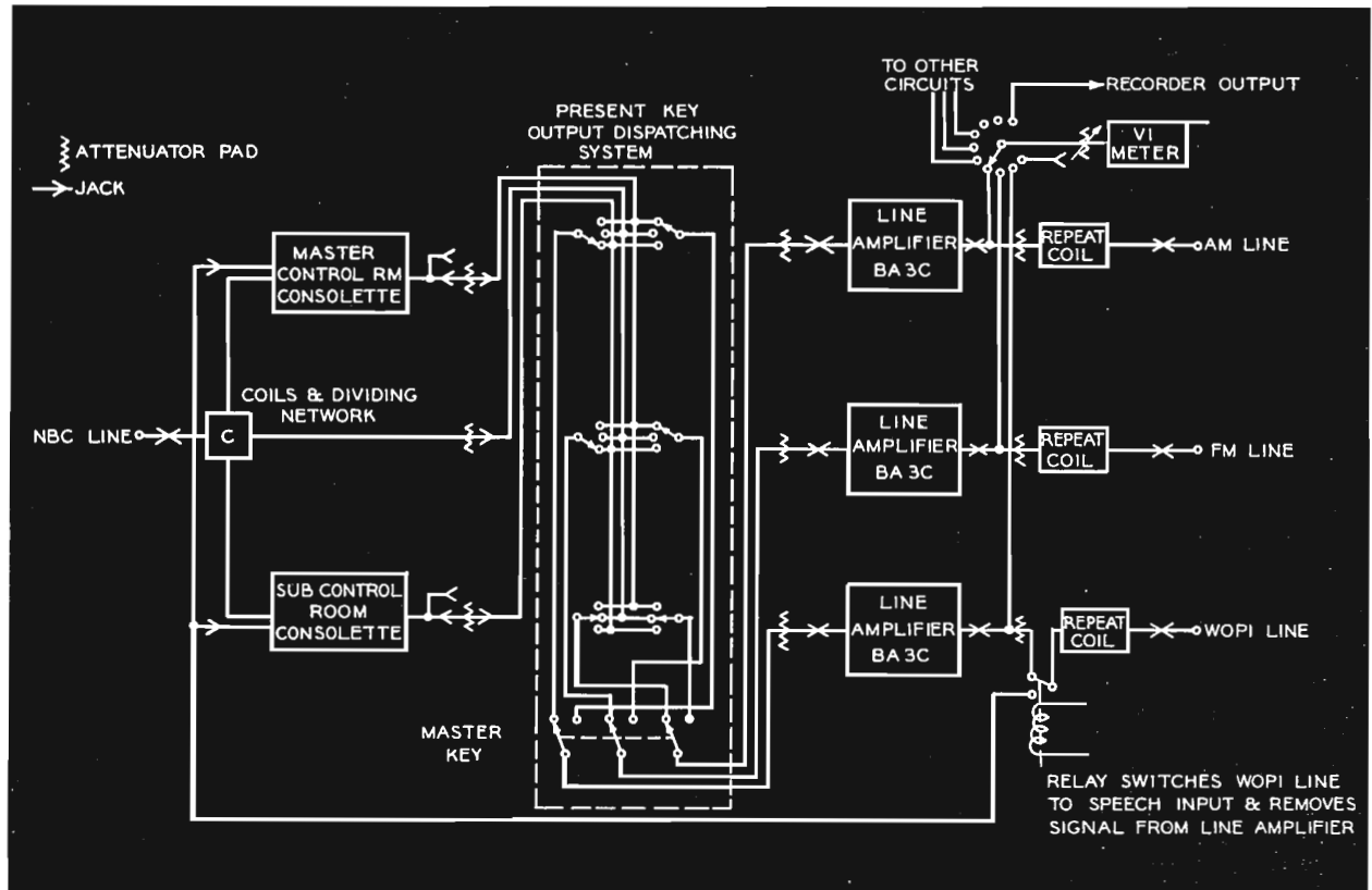
FIG. 6. Simplified schematic diagram showing the program circuit connections for WKPT and WKPT-FM.
