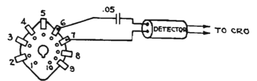
WIRING SIDE
