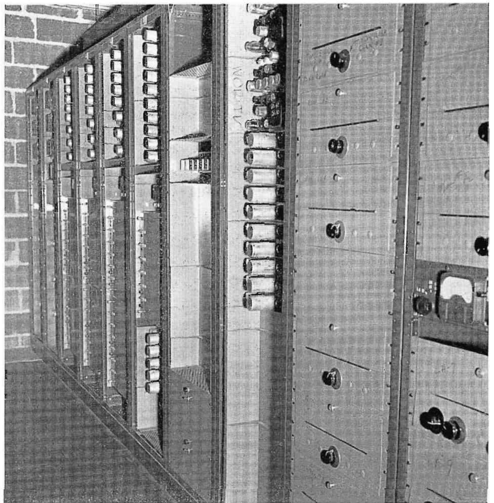
FIG. 37 (above). Second row of Master Control Racks which house TS-20A Video Switching Relays—one rack assigned to each studio system.
