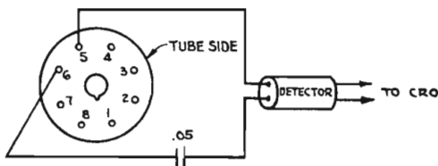
FIG. 9. Socket connections used between Field Camera Control Kinescope (7CP4) and "CRO".
