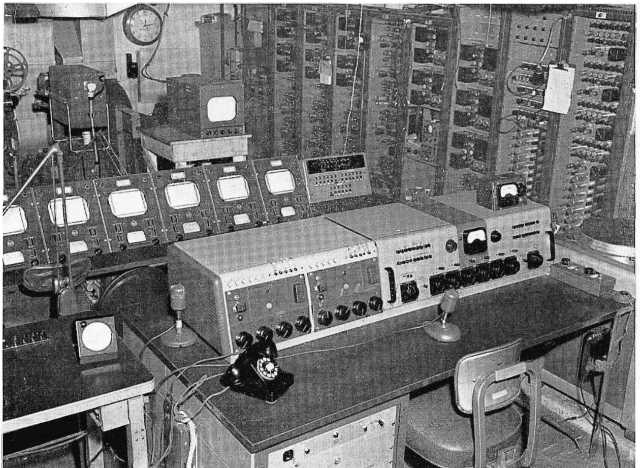
FIG. 42. View of the Program Control Room at the New Amsterdam Theatre. The video console is at a level lower than that of audio console. Sync Generators, Stabilizing Amplifiers and associated equipments are located at the right in fourteen equipment racks.
