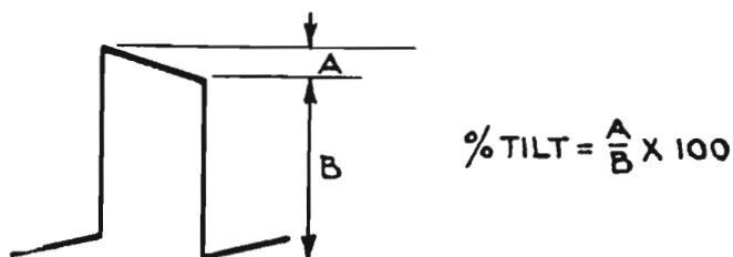
FIG. 15. Square Wave Response of TA-5C Stabilizing Amplifier.
