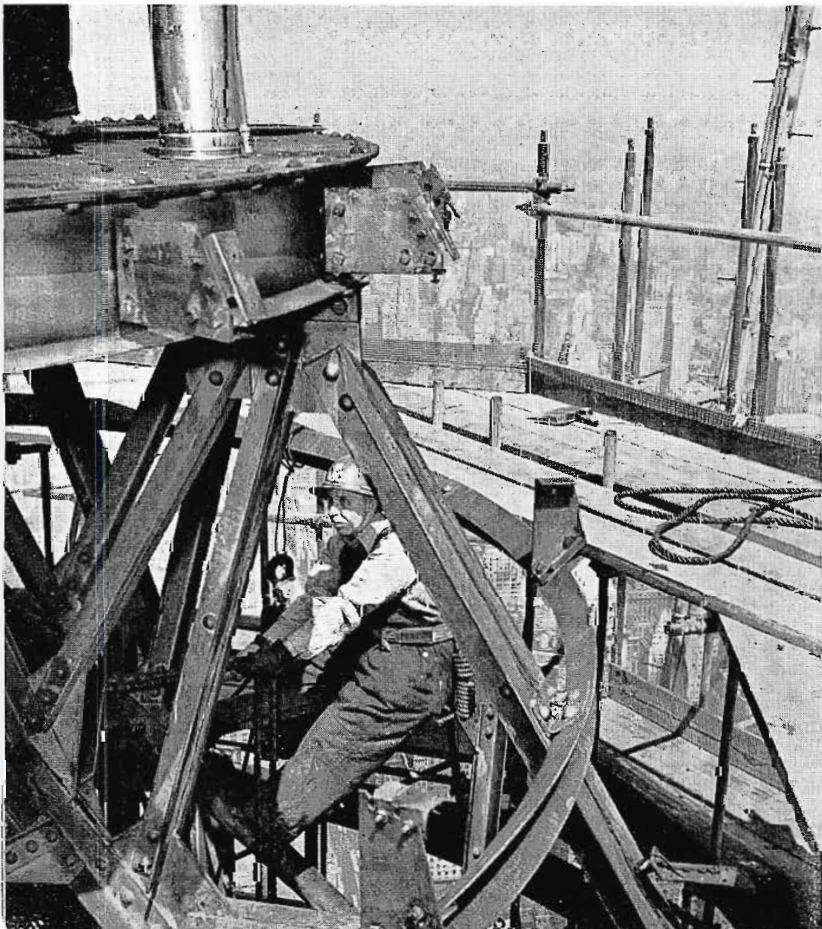
5 Next, after turnstile sections came down, the mammoth job of removing the supporting pole was tackled. (“Spider” Kelly is fastening “rigging” to old tower.) Protective screens avoid falling material and injury.
