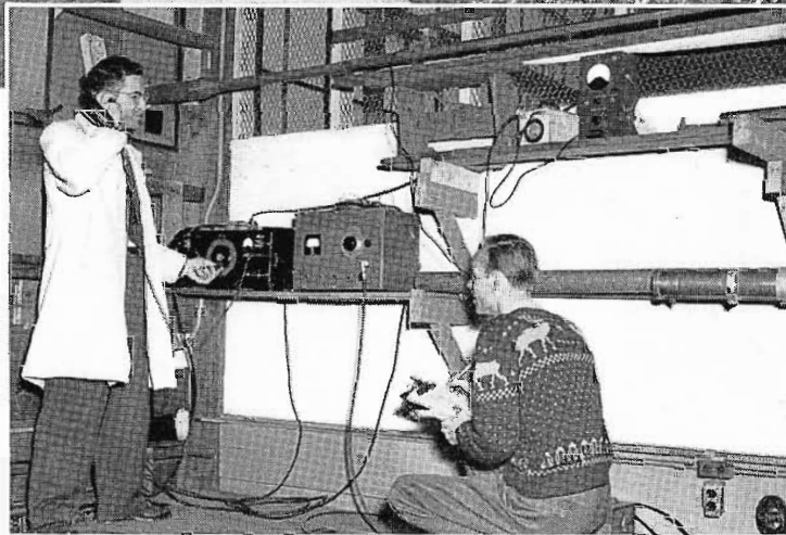
FIG. 5. Richard Wright and Joseph Blake are shown making characteristic impedance measurements on the Super Turnstile Antenna pictured in Fig. 4.
